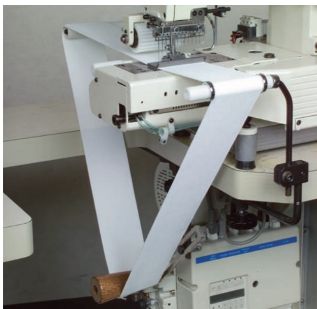
■ RT-1 ゴム張り装置 (手動式) DX, FX (PSF, PMD, PLは除く), RX (RX-P, PLKのみ) RT-1 Elastic expander device ( manual operation ) DX, FX (except for PSF, PMD, PL), RX ( Only for RX-P, PLK ) RT-1 EXPANDIDOR DE ELASTICO DX, FX, RX 松紧带撑开装置 (DX,FX, 除PSF, PMD, PL, RX-P, PLK)
