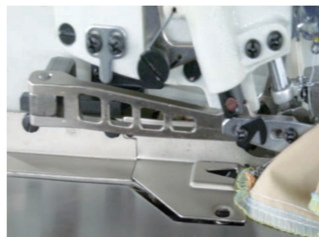
■ HTC 横型空環切り装置 HORIZONTAL CHAIN CUTTER (chain off is cut and is sucked by air horizontally behind the needle plate) CORTADOR DE CADENETA, TIPO HORIZONTAL 横向切线装置
